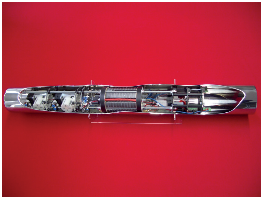
Fig. 1: Complete system without gas supply
