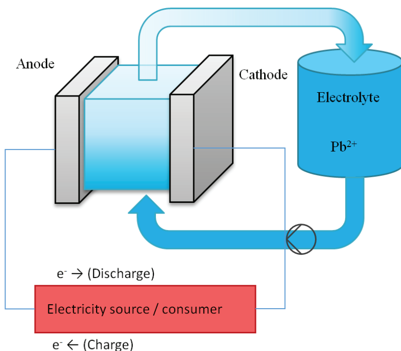
Fig. 1: Diagram of the SLFB
