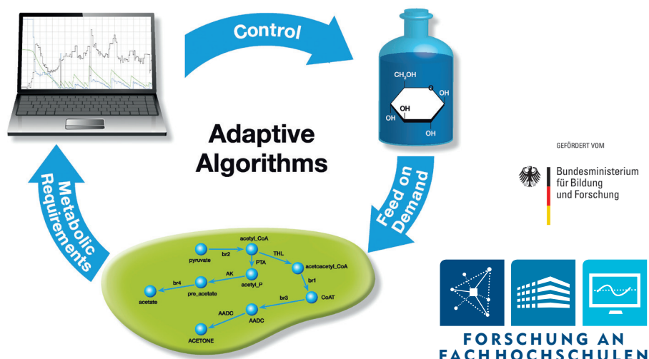
Fig. 1: Adaptive Algorithms
