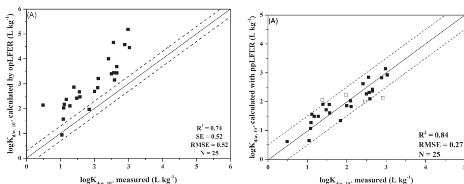
Fig. 1: Comparison of the spLFER-Approach (left) with \log K_{o/w} to the ppLFER-Approach (right). The illustrations show the calculated logarithmic distribution coefficients ( \log K_{d/w} ) against the actually measured logarithmic distribution coefficients. A clear improvement can be seen in the ppLFER model compared with the spLFER model in relation to the coefficient of determination ( R^2 ), and the root of the mean square of error (RMSE).
