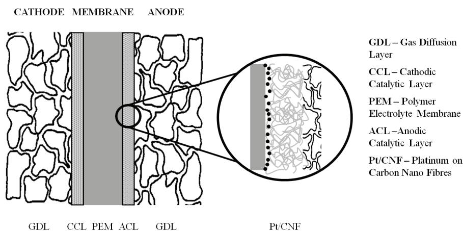
Fig. 1: Diagram of a membrane electrode unit for PEM-fuel cells (cross-section)
