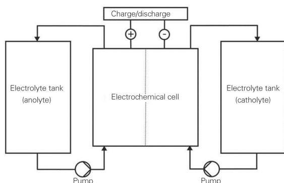
Fig. 1: Schematic Sketch of a Redox-Flow Battery
