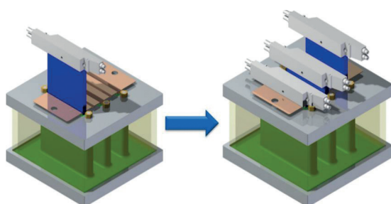
Fig. 2: Schematic Construction of a Modular Stack in Pocket Construction
